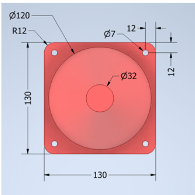
Figure 8.2 Pylon Top View
