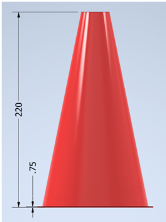
Figure 8.1 Pylon Side View (all thicknesses are 0.75 mm)
