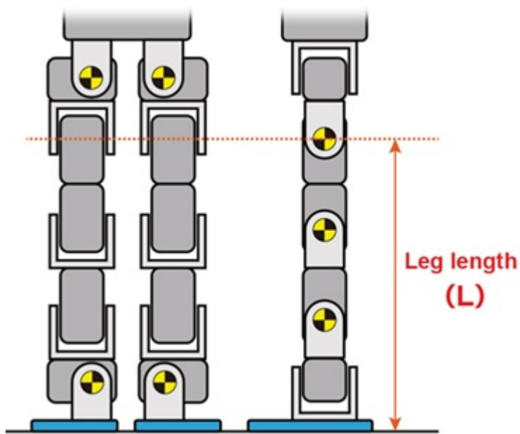
Figure 5-5 Leg length
